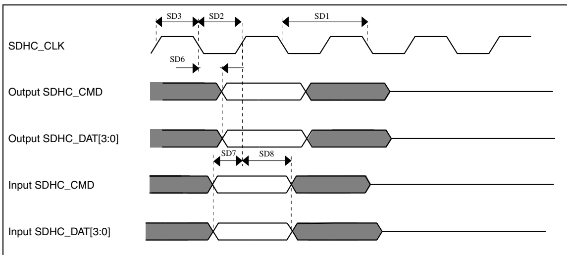
Figure 53. SDHC timing
