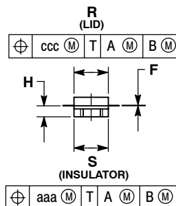
CASE 360C-05 ISSUE D NI-360S MRF9030LSR1
