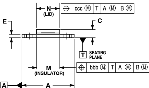
CASE 360B-05 ISSUE F NI-360 MRF9030LR1
