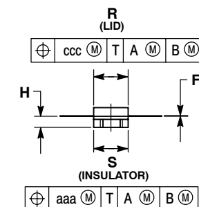
CASE 360B-05 ISSUE F NI-360 MRF9030LR1
