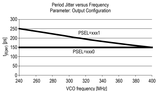
Figure 7. Max. Period Jitter versus VCO Frequency
