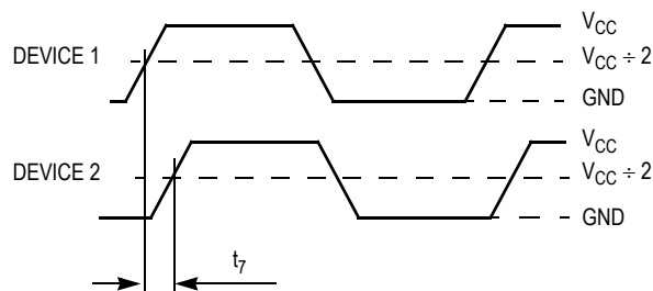
Figure 4. Device-to-Device Skew
