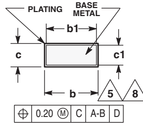
SECTION F-F
