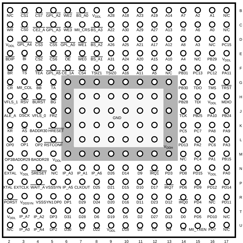
Figure 63. Pinout of the PBGA Package - non-JEDEC
