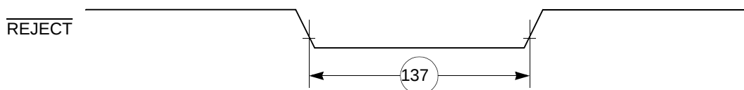
Figure 53. CAM Interface \overline{\text{REJECT}} Timing Diagram
