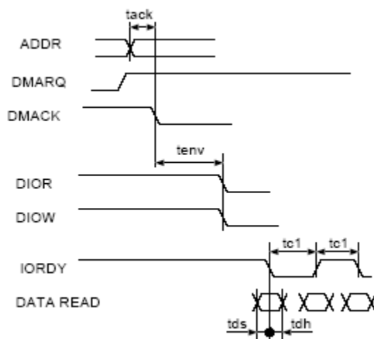
Figure 72. UDMA in Transfer Starts Timing Diagram
