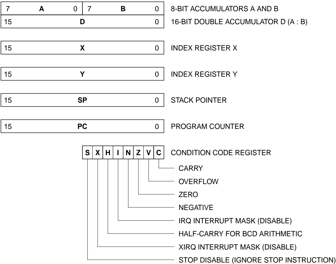
Figure 10 Programming Model
