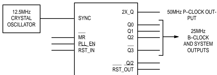
Figure 5. Logical Representation of the MC88920 With Input/Output Frequency Relationships
