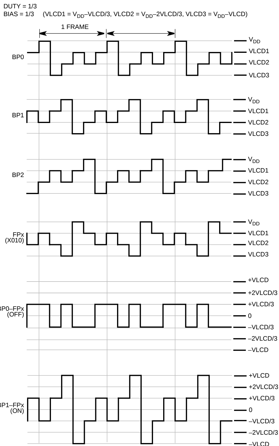
Figure 10-3. LCD 1/3 Duty and 1/3 Bias Timing Diagram
