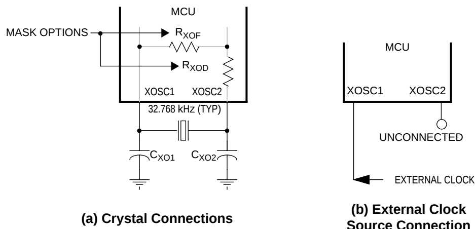
Figure 1-4. Oscillator Connections
