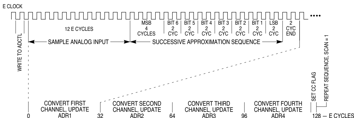
Figure 7-1 A/D Conversion Sequence
