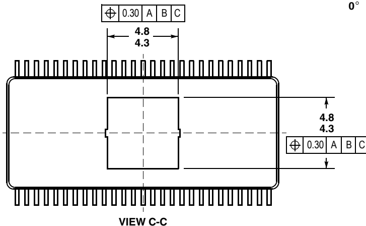
VIEW C-C
