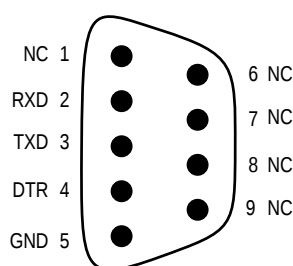
Figure 2-9. Host Computer to JLJKICS Interconnection (J4)
