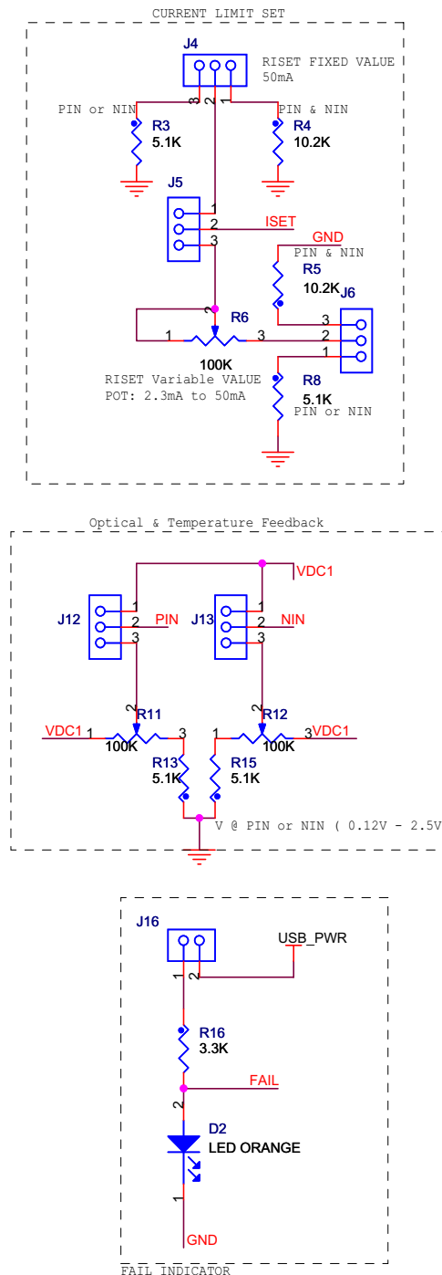
Figure 10. EVB Schematic (3)
