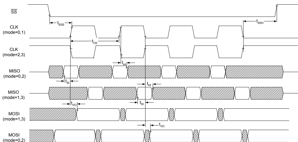
Figure 42: SPI Timing (Master)
