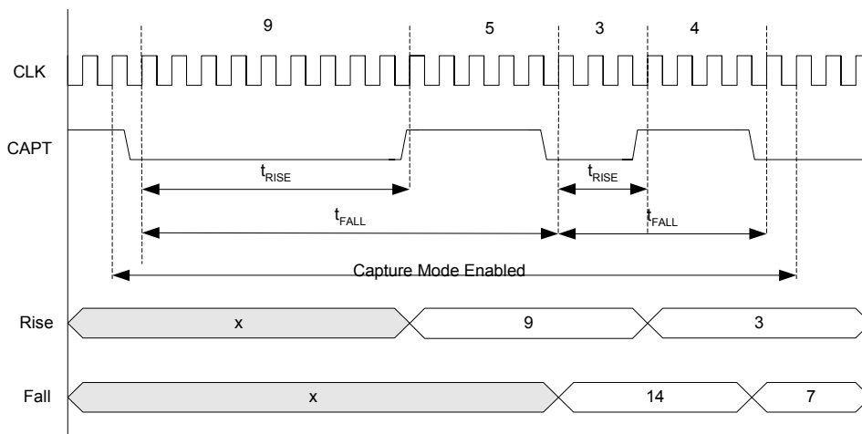
Figure 28: Capture Mode
