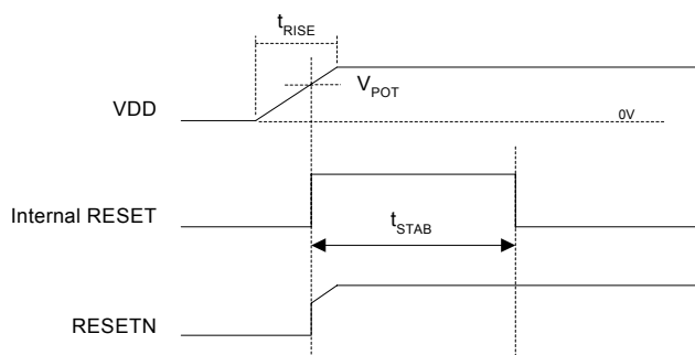
Figure 40: Power-on Reset
