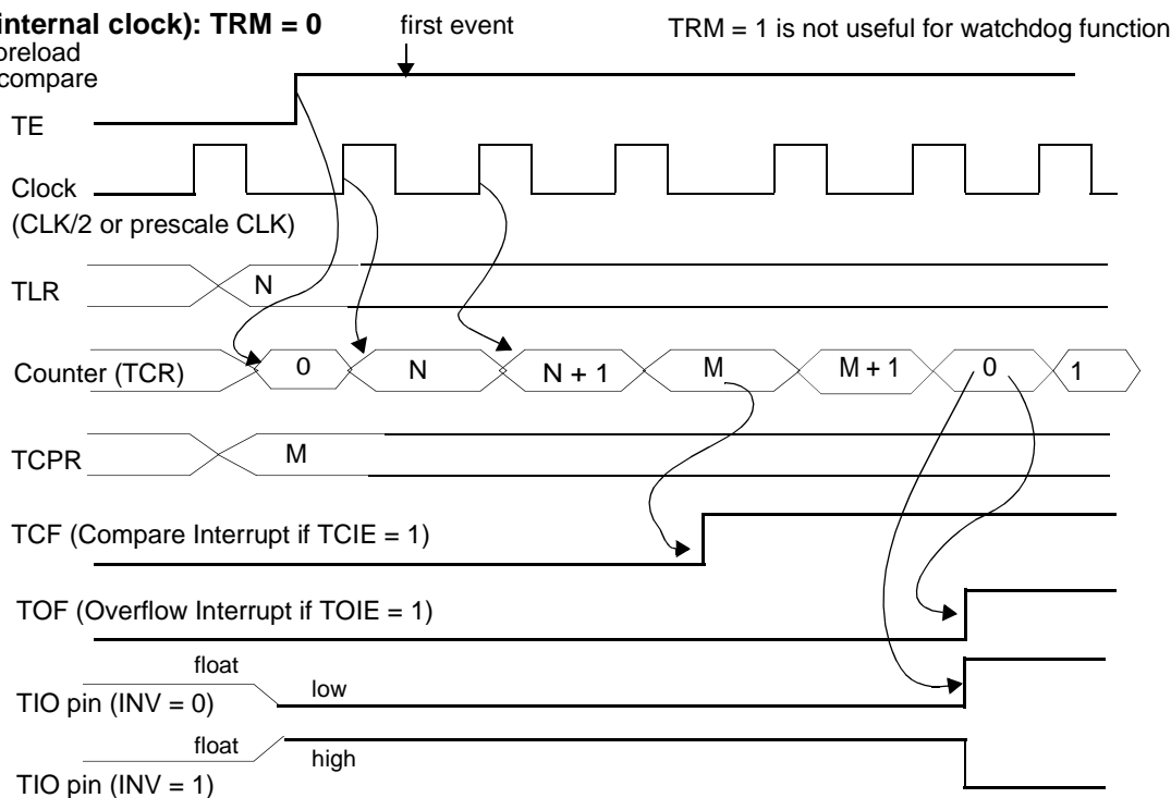
Figure 9-19. Watchdog Toggle Mode
