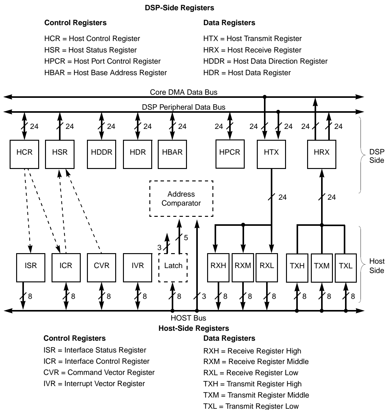
Figure 6-1. HI08 Block Diagram
