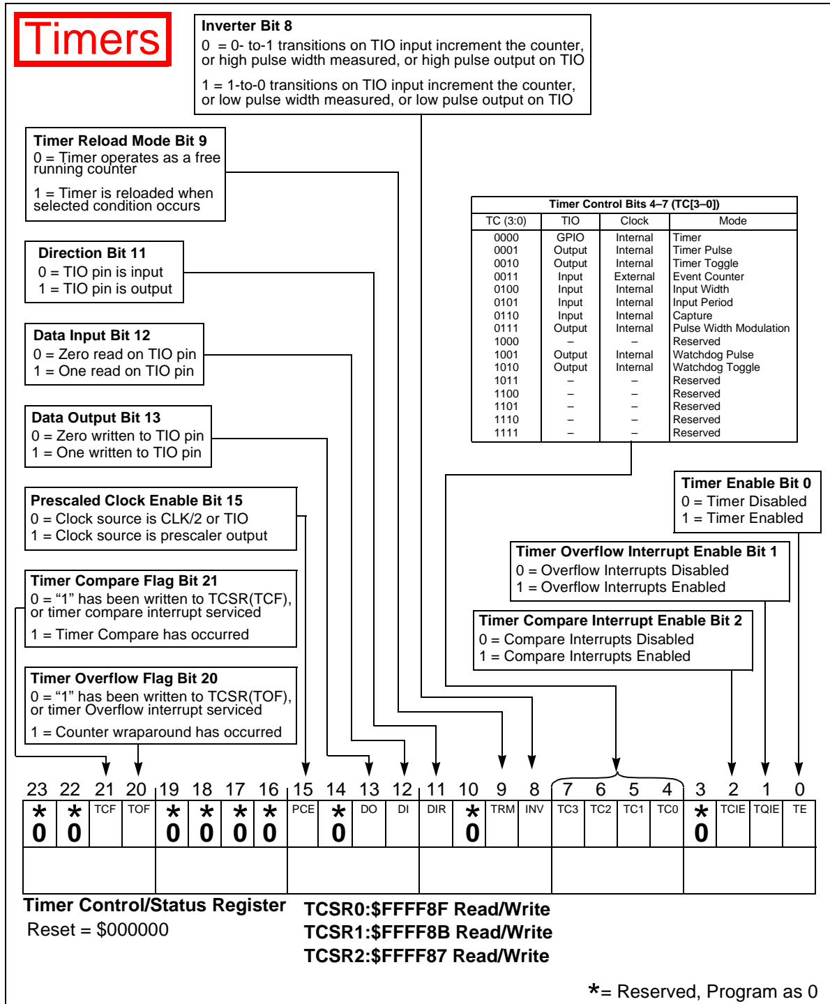
Figure B-21. Timer Control/Status Register (TCSR)
