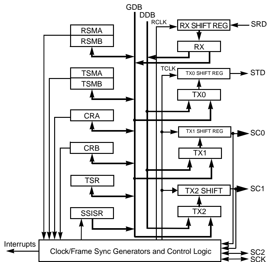
Figure 7-1. ESSI Block Diagram
