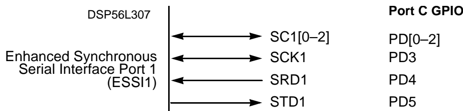
Figure 5-4. Port D Signals
