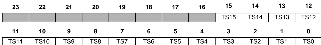
Figure 7-14. ESSI Transmit Slot Mask Register A (TSMA)
