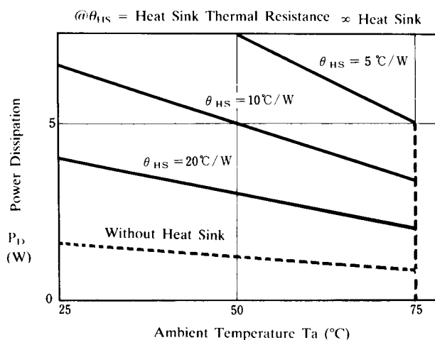
NJM2930 (TO-220F)
