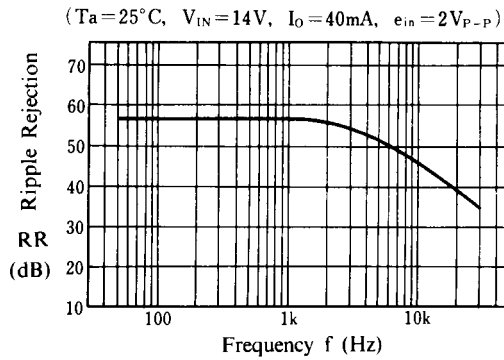
NJM2930F05/L05 Ripple Rejection vs. Frequency
