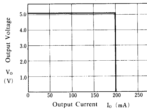
NJM2930F05/L05 Load Characteristics
