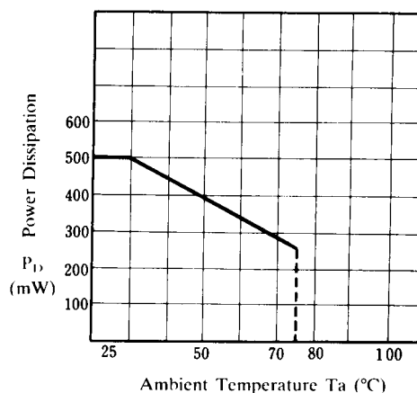
NJM2930L (TO-92)
