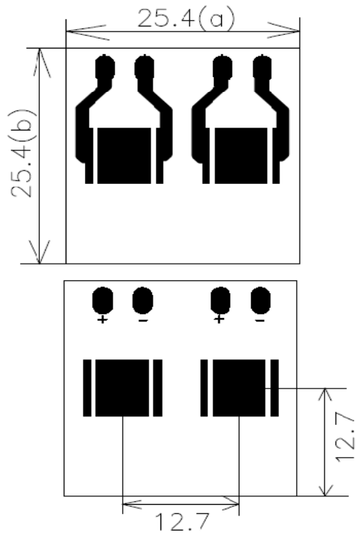
1" SQUARE MCPCB
