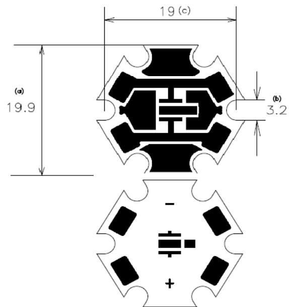
STAR MCPCB
