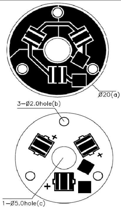
Round 3LED MCPCB White mask Black letter
