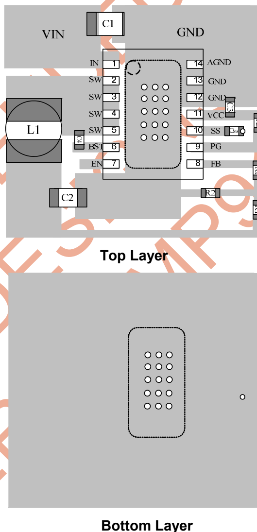
Figure 7—PCB Layout
