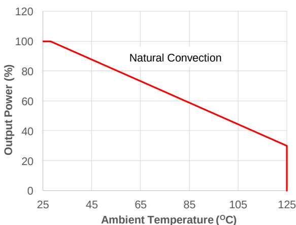
Power Derating VIN = 12V, VOUT = 1V
