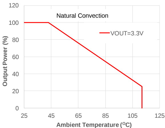
Power Derating V_{IN} = 12V , V_{OUT} = 3.3V
