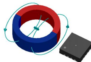
Figure 5: Side-Shaft Mounting
