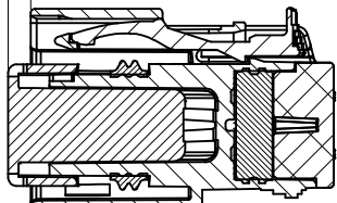
PRIMARY LOCK REINFORCEMENT (PLR) SHOWN IN PRE-STAGED POSITION SECTION Y-Y
