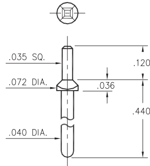
8953-0-05-XX-00-00-03-0 Square press-fit in .047 plated thru hole
