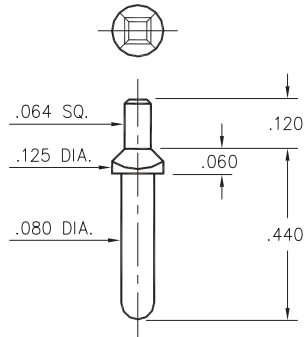
8952-0-05-XX-00-00-03-0 Square press-fit in .087 plated thru hole
