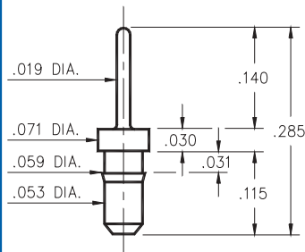
8876-0-00-XX-00-00-03-0 Press-fit in .057 mounting hole
