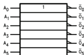
IEEE / IEC LOGIC SYMBOL
