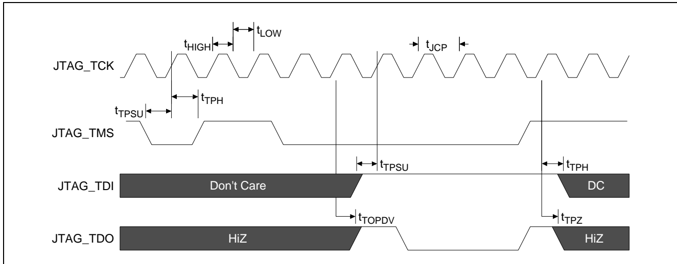
Figure 31 - JTAG Signal Timing
