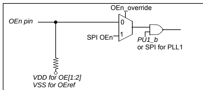
Figure 7 - Output Enable/Disable
