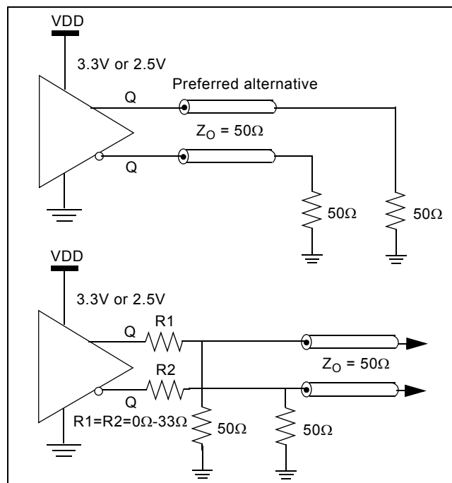
Figure 15 - HCSL Output Loads &amp; Test Circuits
