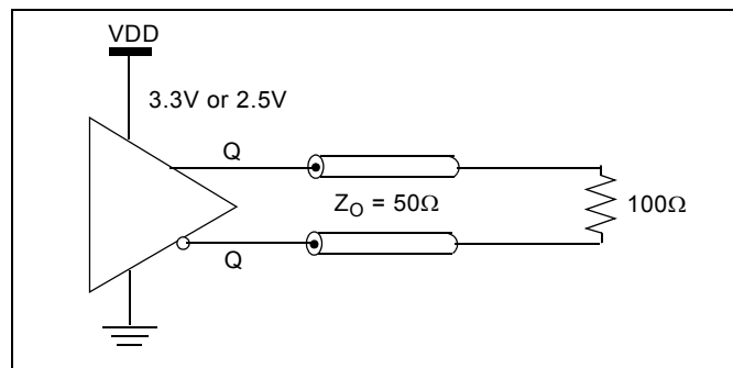
Figure 12 - LVDS Output Load &amp; Test Circuit
