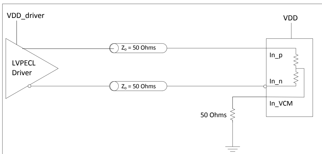
Figure 5 - Input Termination - LVPECL DC coupled
