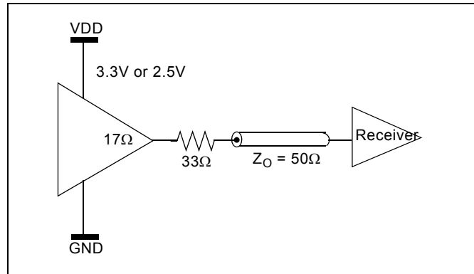
Figure 13 - LVCMOS Output Load &amp; Test Circuit
