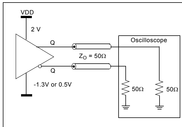
Figure 14 - LVPECL Output Load &amp; Test Circuit
