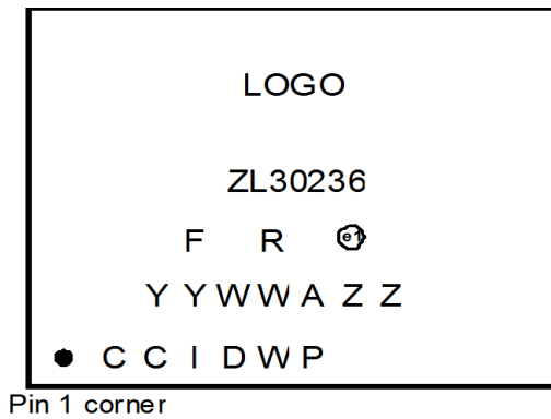
Figure 28 - Custom Factory Programmed Device Top Mark
