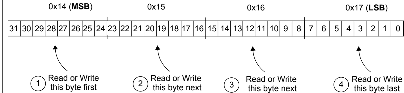
Figure 23 - Accessing Multi-byte Register Values
