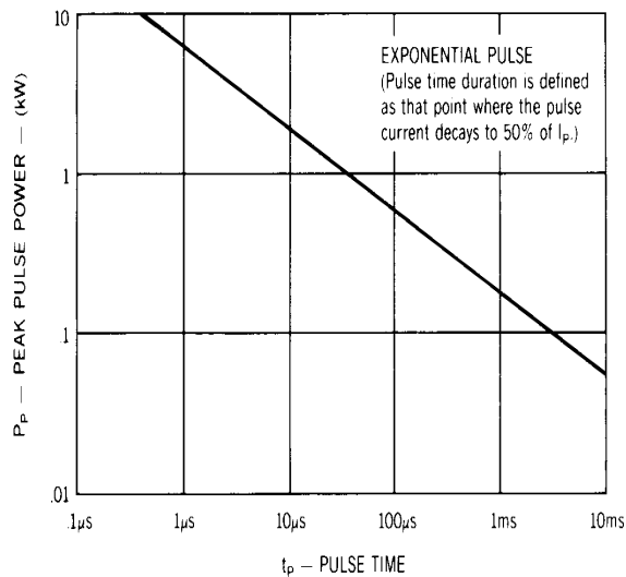
Figure 2. Peak Pulse Power vs. Pulse Duration
