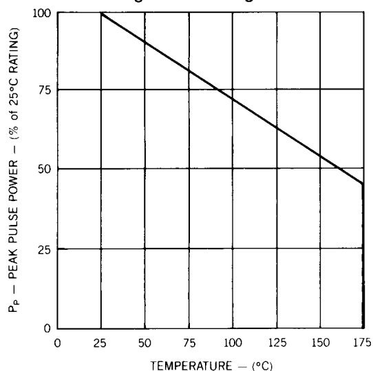
Figure 3. Derating Curve
