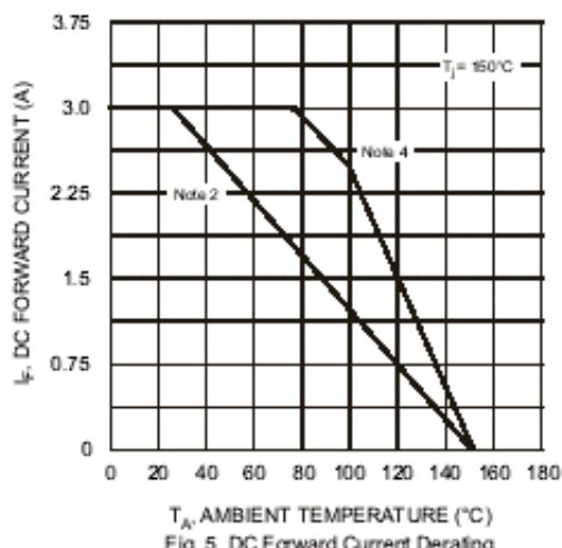
Fig. 5 DC Forward Current Derating
