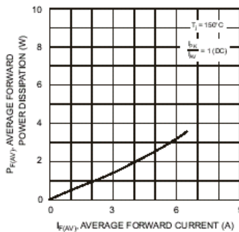
Fig. 6 Forward Power Dissipation
