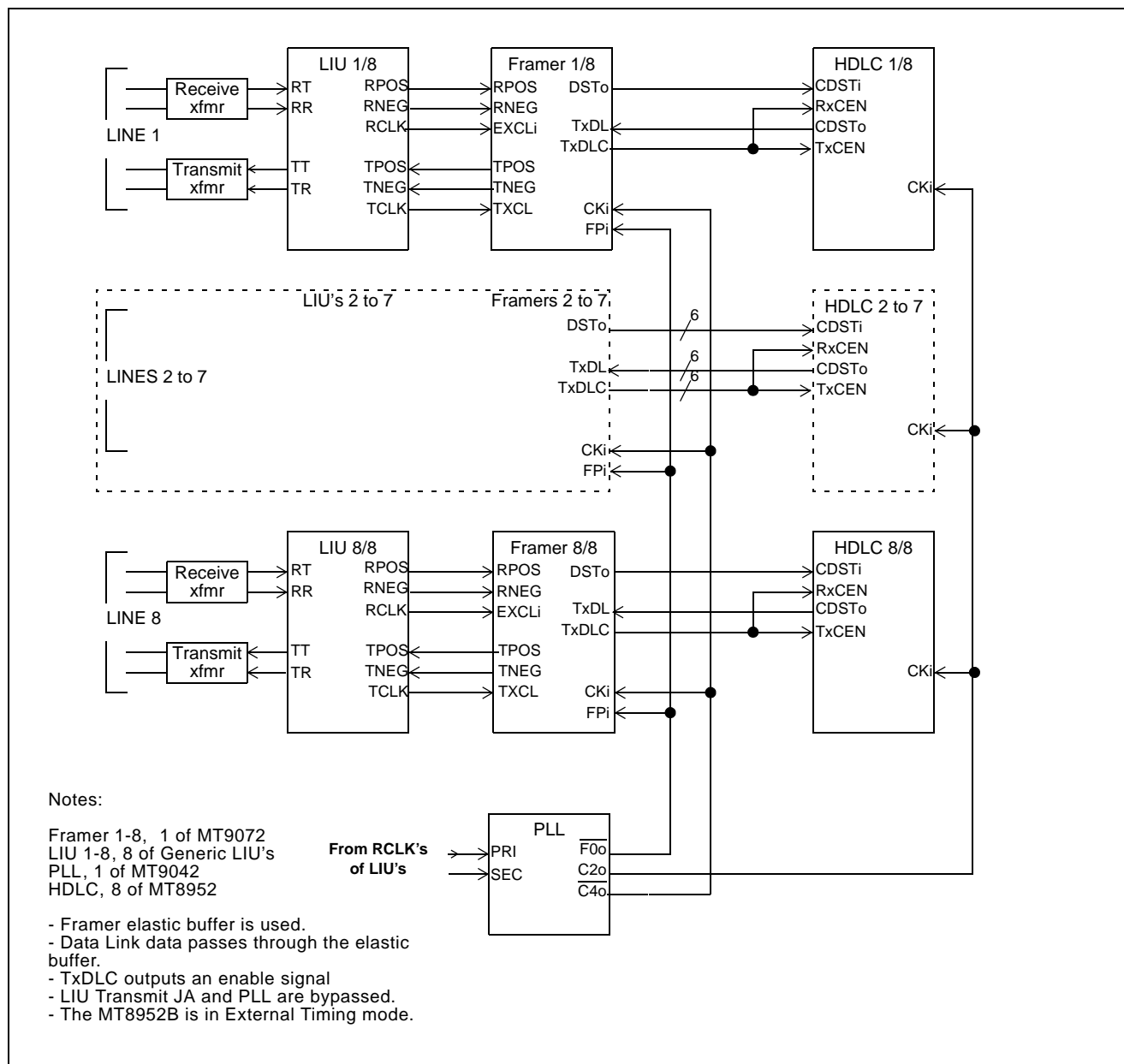
Figure 12 - 8 T1 Links with Synchronous Data Link Signaling
