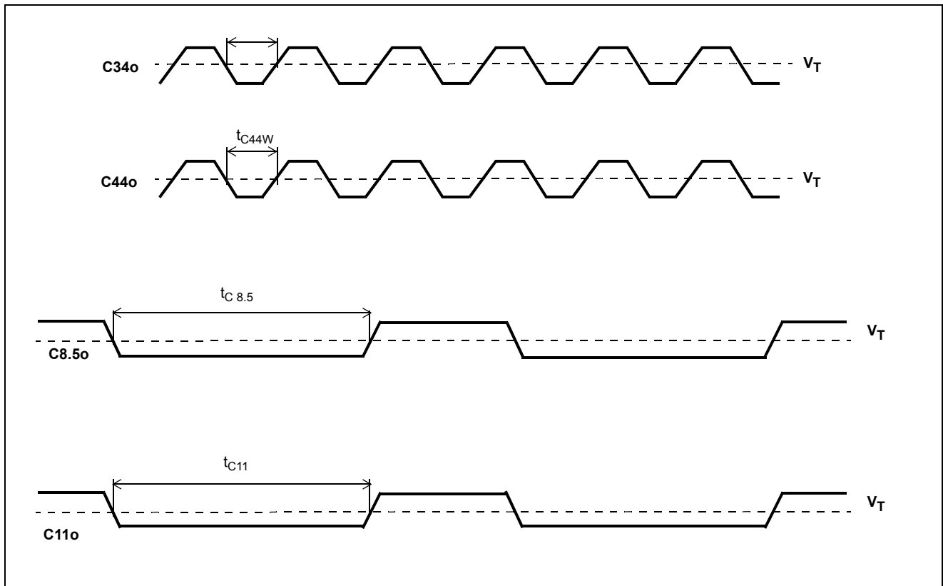
Figure 21 - Output Timing 3
