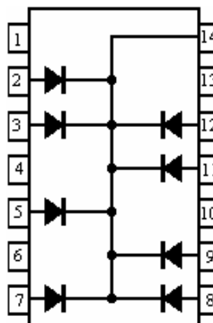
CIRCUIT CONFIGURATION
