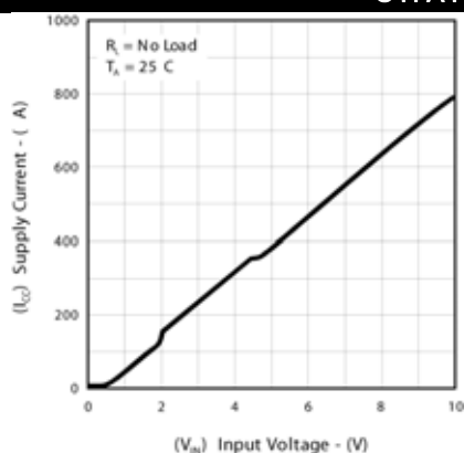
Figure 7 – Supply Current vs. Input Voltage
