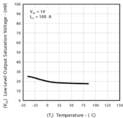
Figure 11 – Low Level Output Saturation Voltage vs. Temperature
