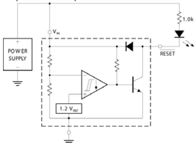
Figure 17 – Voltage Monitor
