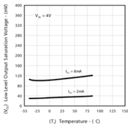
Figure 10 – Low Level Output Saturation Voltage vs. Temperature
