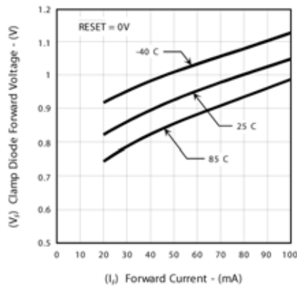
Figure 12 – Clamp Diode Forward Voltage vs. Forward Current
