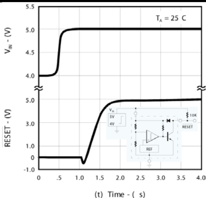
Figure 14 – Propagation Delay – LOW to HIGH
