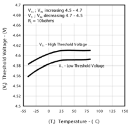
Figure 5 – Threshold Voltage vs. Temperature
