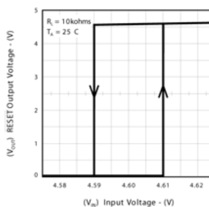
Figure 4 – \overline{\text{RESET}} Output Voltage vs. Input Voltage
