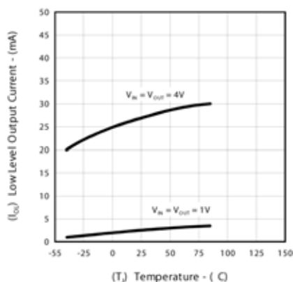
Figure 9 – Low Level Output Current vs. Temperature
