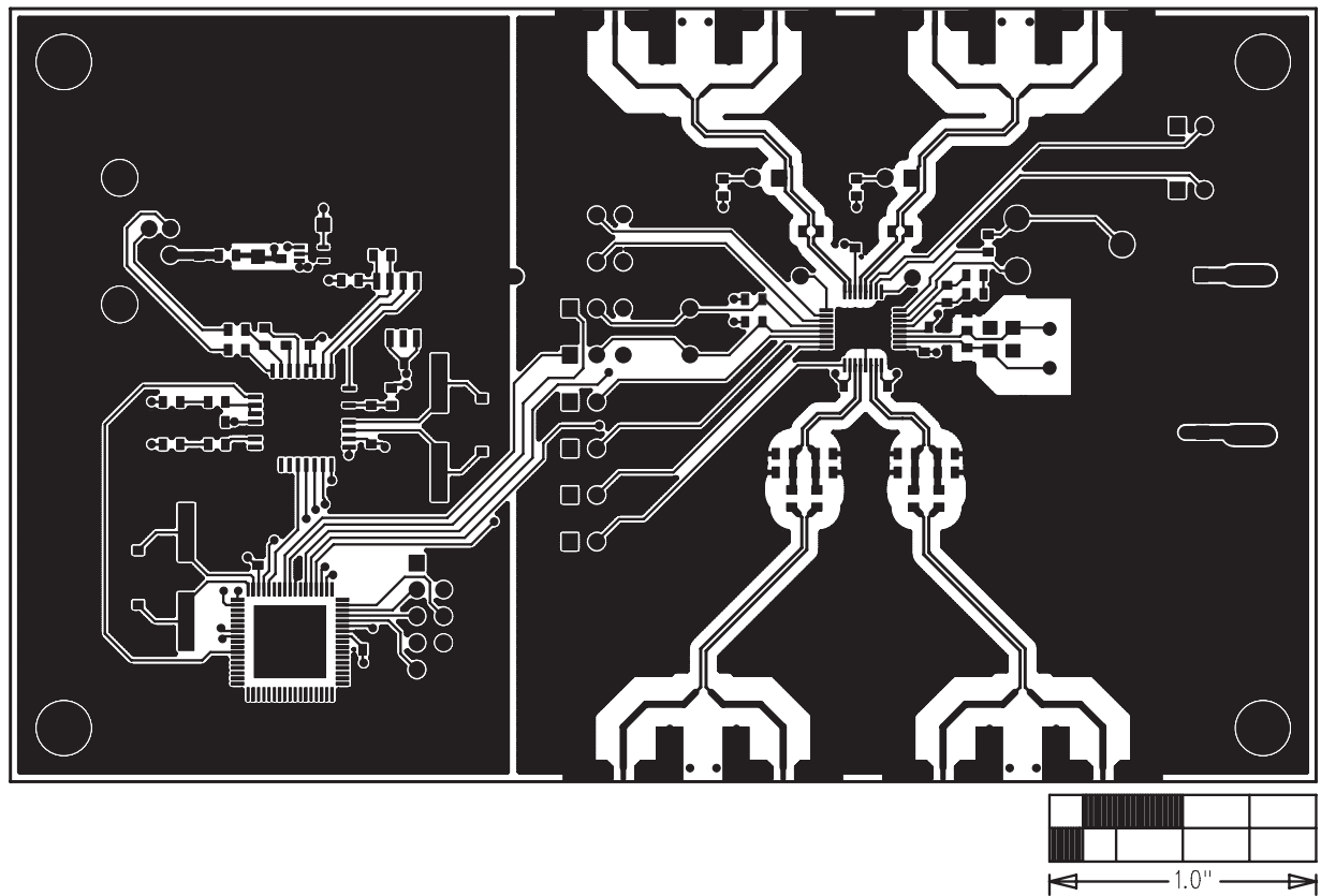
Figure 8. MAX9451 EV Kit PCB Layout—Component Side
