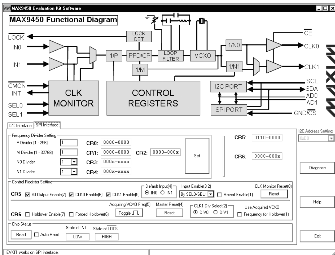
Figure 4. MAX9450 EV Kit Software—SPI Interface Tab
