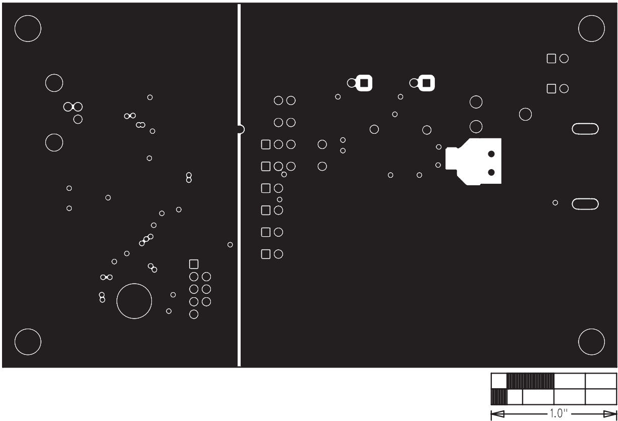
Figure 9. MAX9451 EV Kit PCB Layout—Ground Plane
