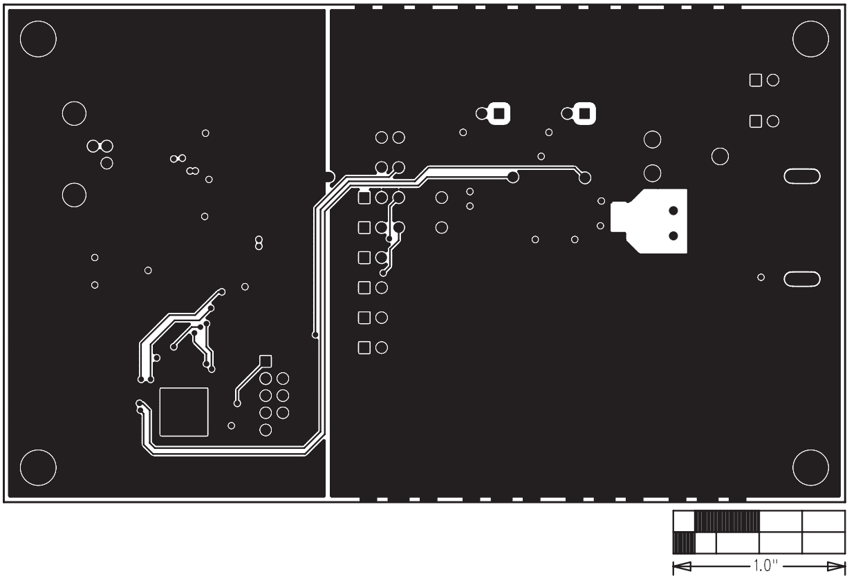
Figure 11. MAX9451 EV Kit PCB Layout—Solder Side
