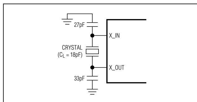
Figure 6. Crystal, Capacitors Connection
