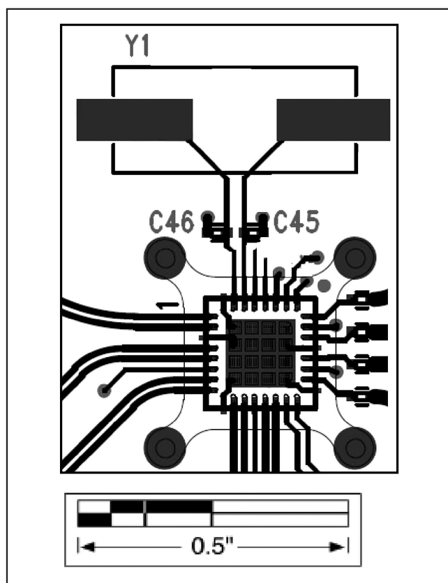
Figure 5. Crystal Layout
