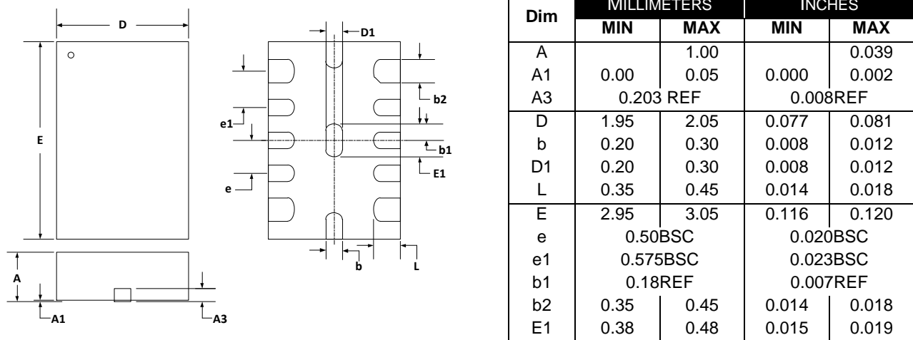
Figure 8 · LQ 12-Pin VQFN Package Dimensions
