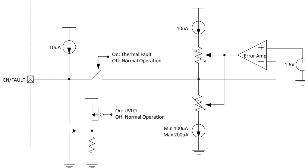
Figure 6 · Simplified EN/FAULT circuitry
