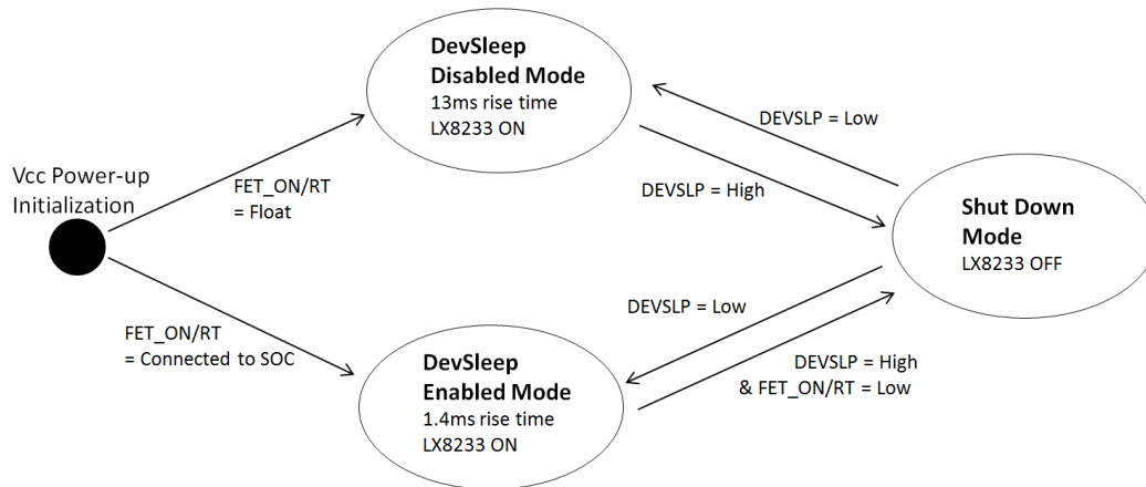
Figure 5 · DevSleep Operation
