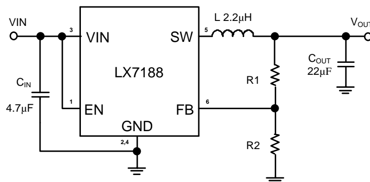
Figure 11 · Typical Application
