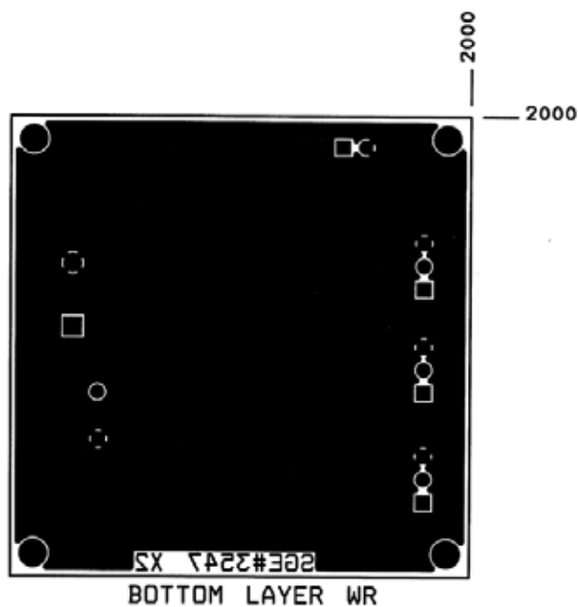
Figure 3 – LX2208 Evaluation Board Layout
