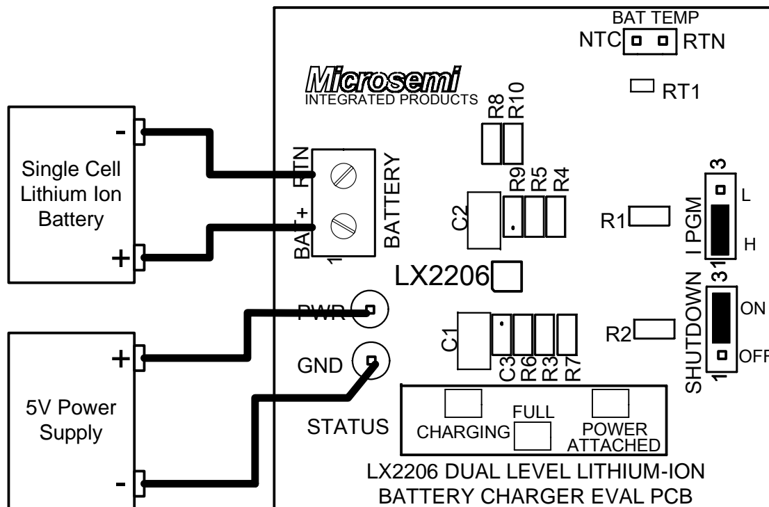
Figure 3 – LX2206 Typical Test Hookup
