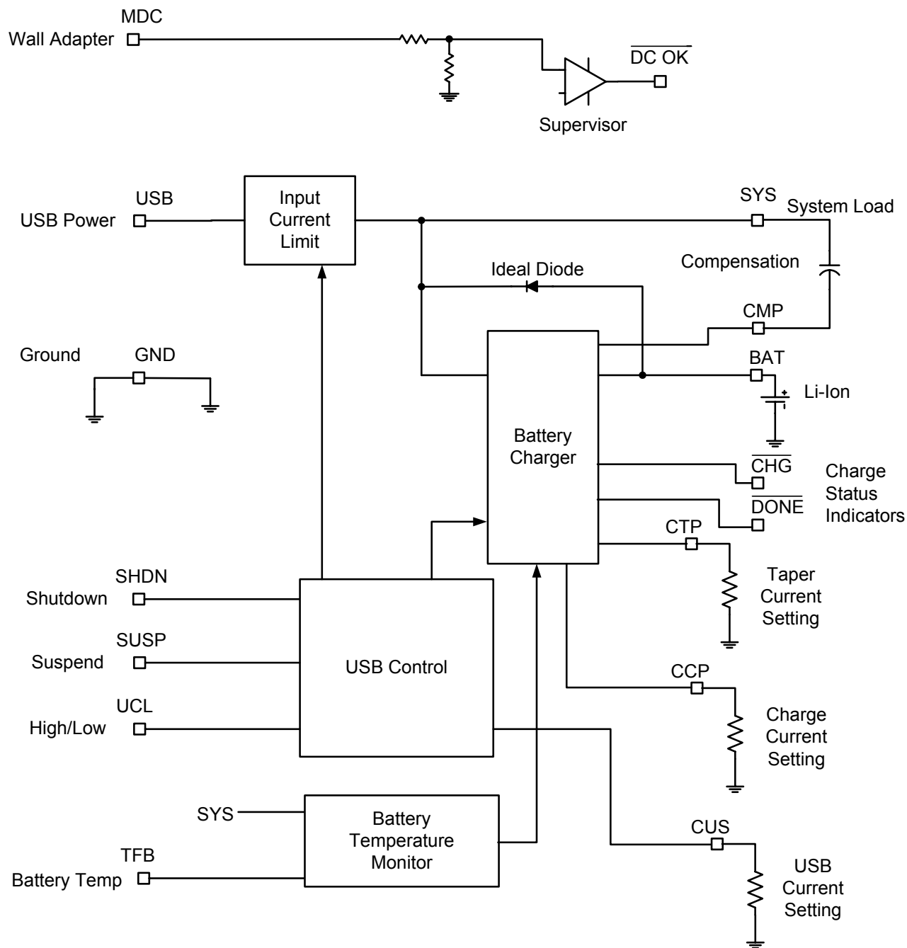
Figure 2 – Simplified Block Diagram
