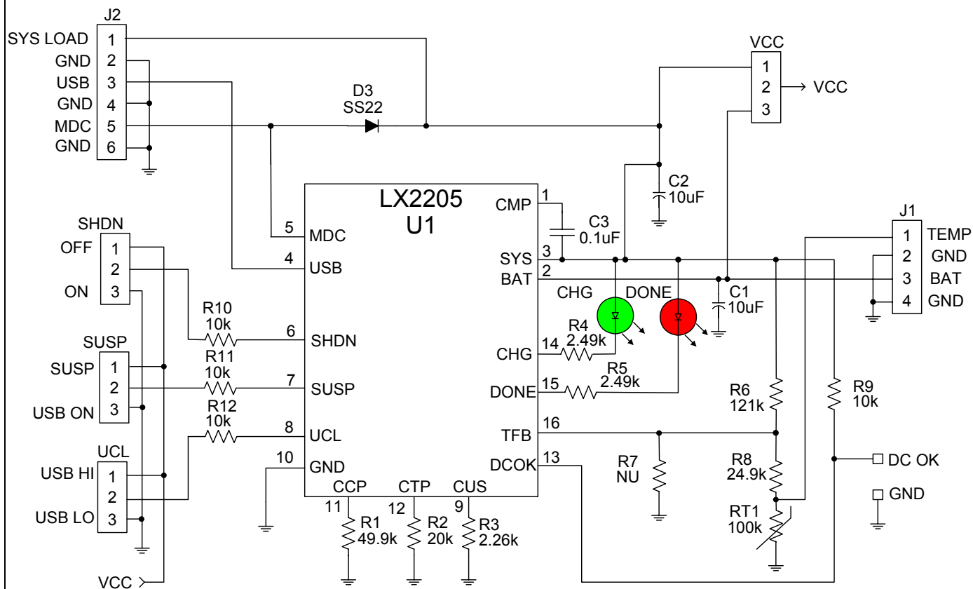
Figure 1 – LX2205 Evaluation Board Schematic
