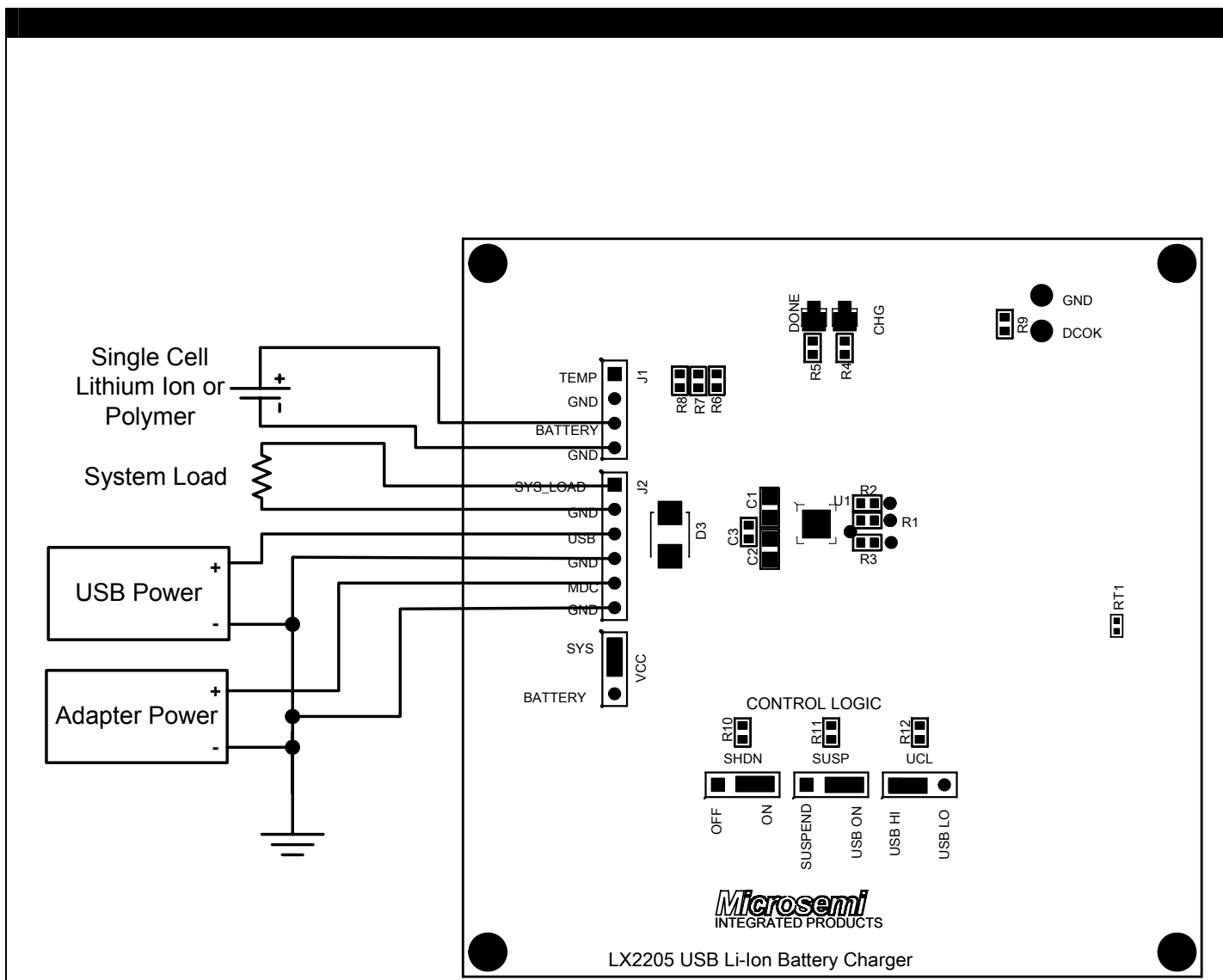
Figure 3 – LX2205 Typical Test Hookup
