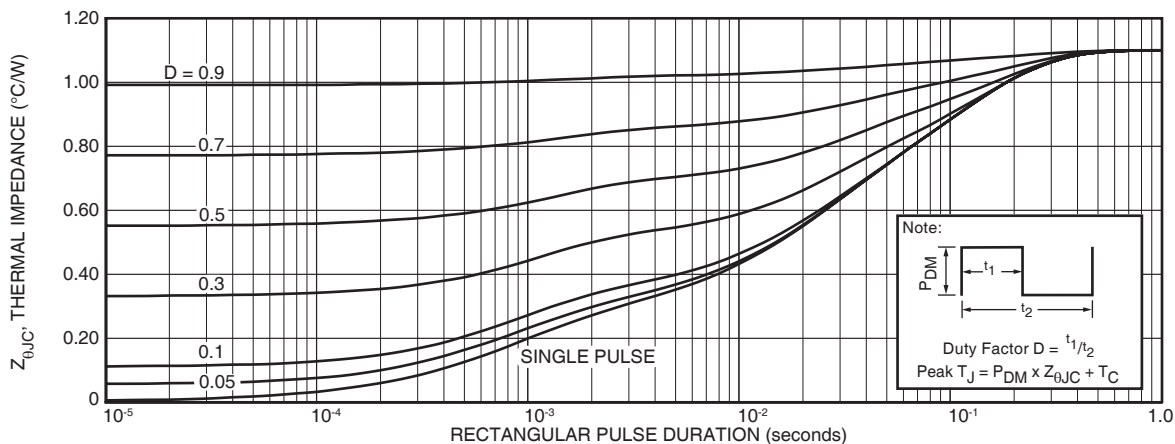
FIGURE 24a. MAXIMUM EFFECTIVE THERMAL IMPEDANCE, JUNCTION-TO-CASE vs. PULSE DURATION
