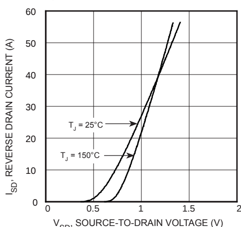
FIGURE 8, Reverse Drain Current vs Source-to-Drain Voltage
