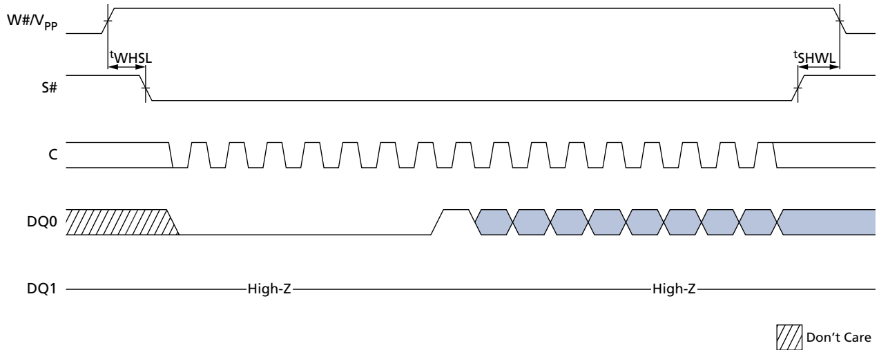
Figure 37: Hold Timing
