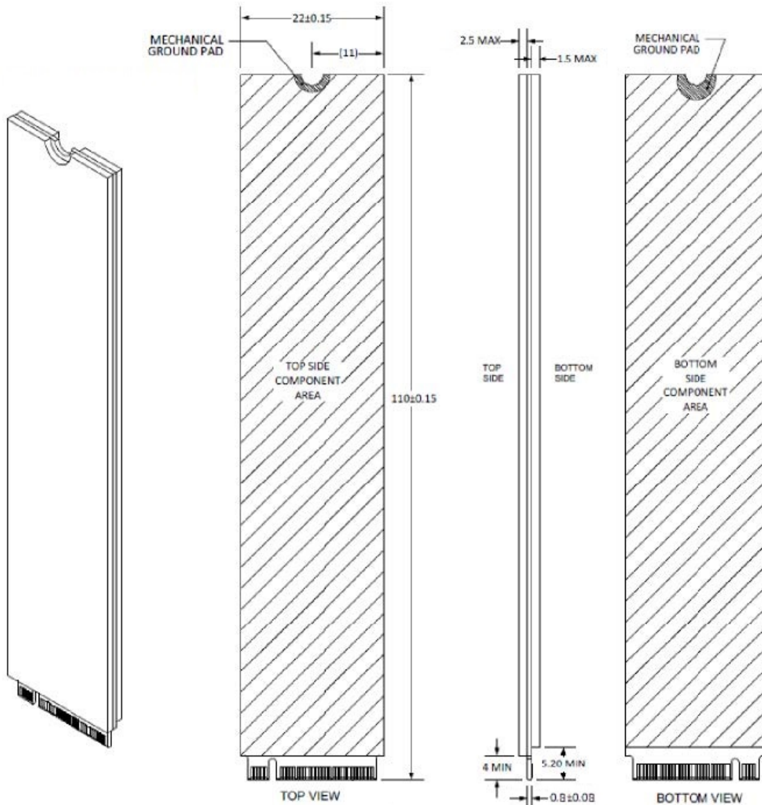
Figure 4: Nominal Dimensions
