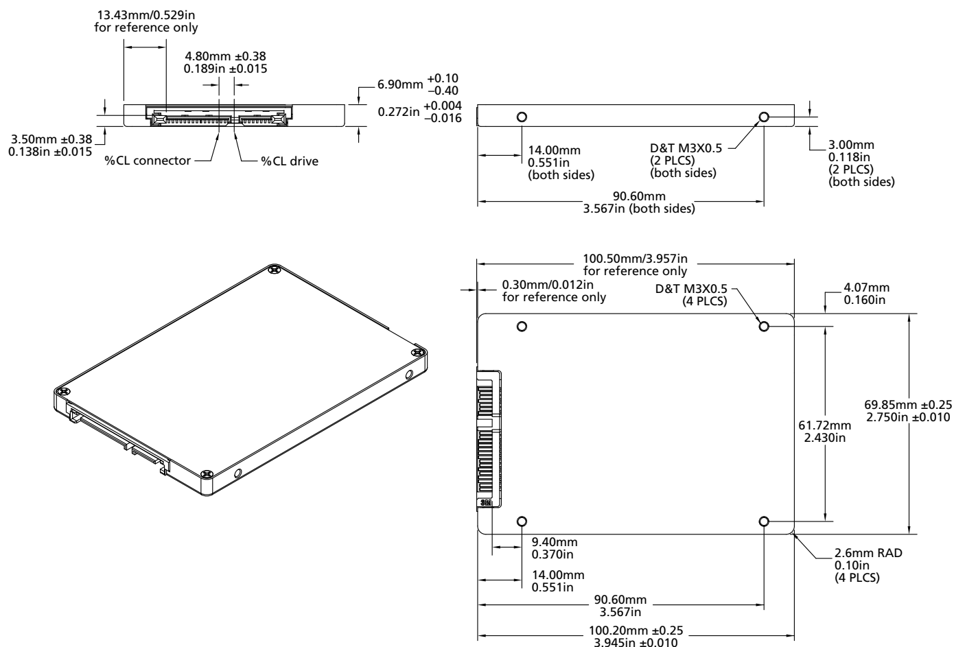
Figure 4: 2.5-Inch Package – 7mm
