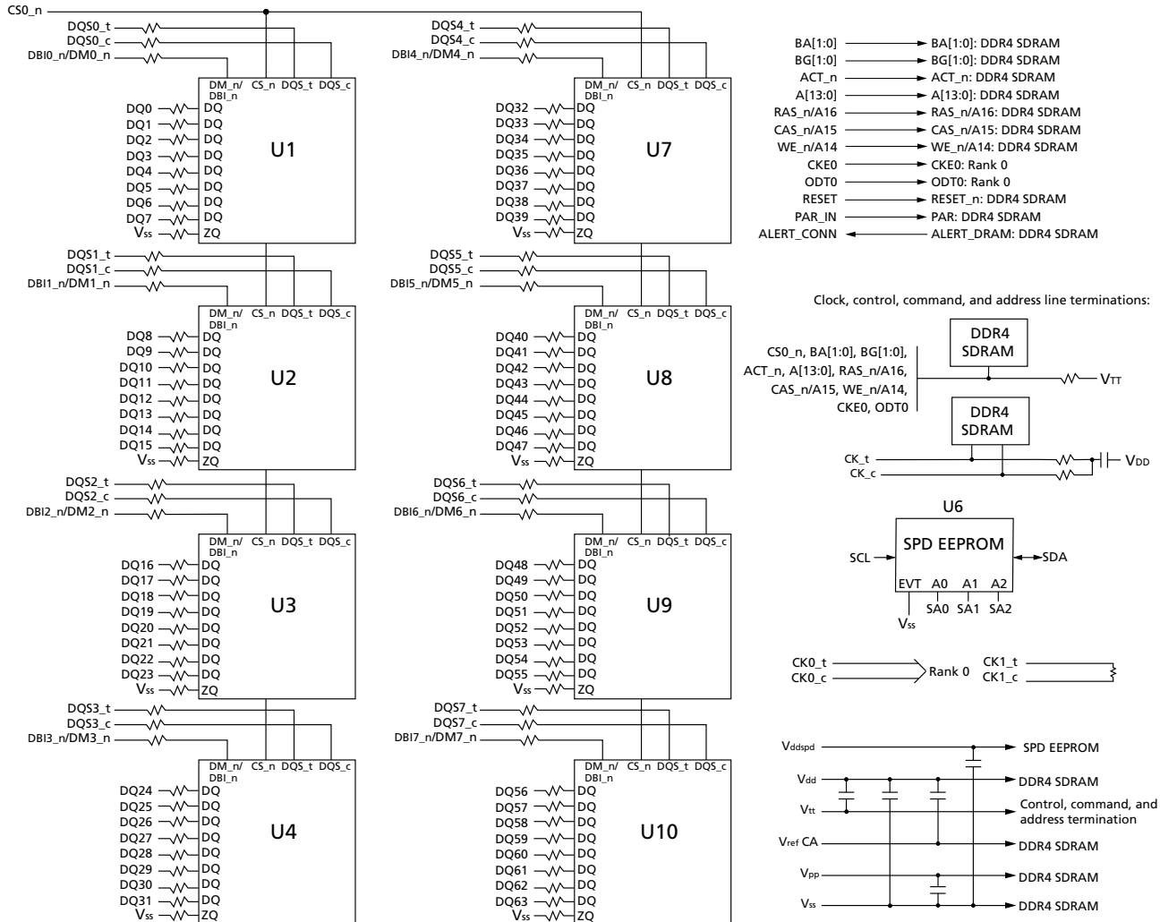
Figure 2: Functional Block Diagram (R/C-A1)
