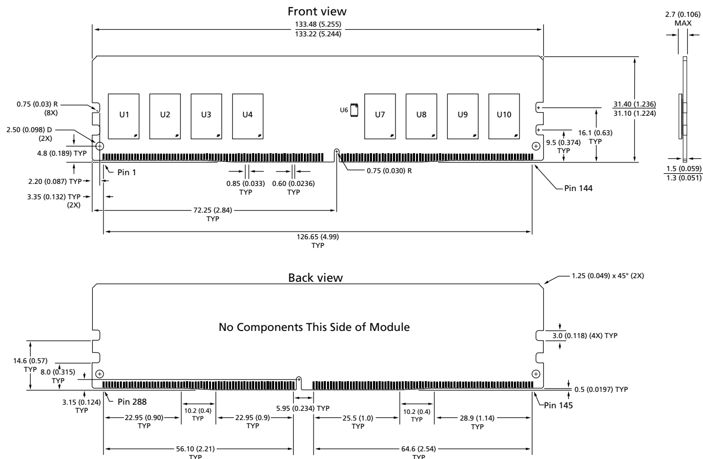
Figure 3: 288-Pin DDR4 UDIMM (R/C-A1)
